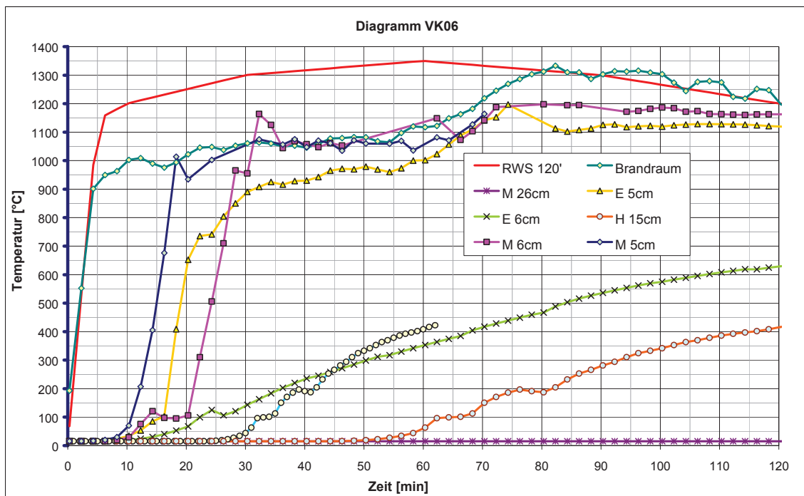
Abb. 6: Sondentemperaturen VK06
