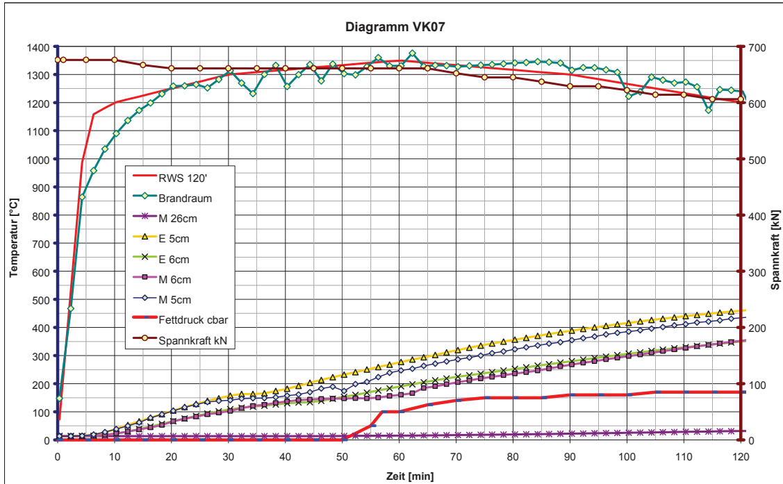
Abb. 7: Sondentemperaturen VK07
